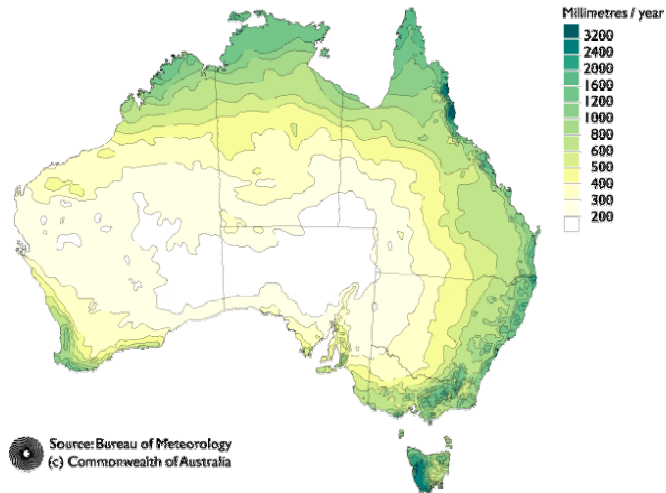
Figure 3: Average annual rainfall based on 30-year climatology (1961-1990)
