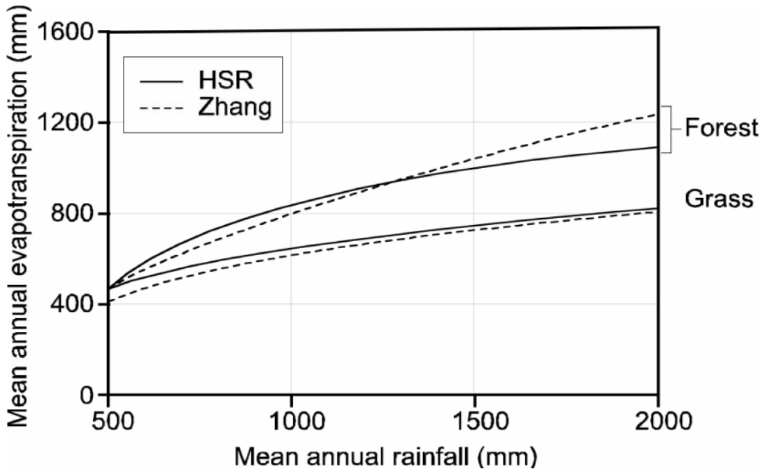
Figure 6: Relationship between land cover, mean annual rainfall and mean annual evapotranspiration, as predicted by Holmes and Sinclair (1986) and Zhang (1999). In Keenan et al 2004.
