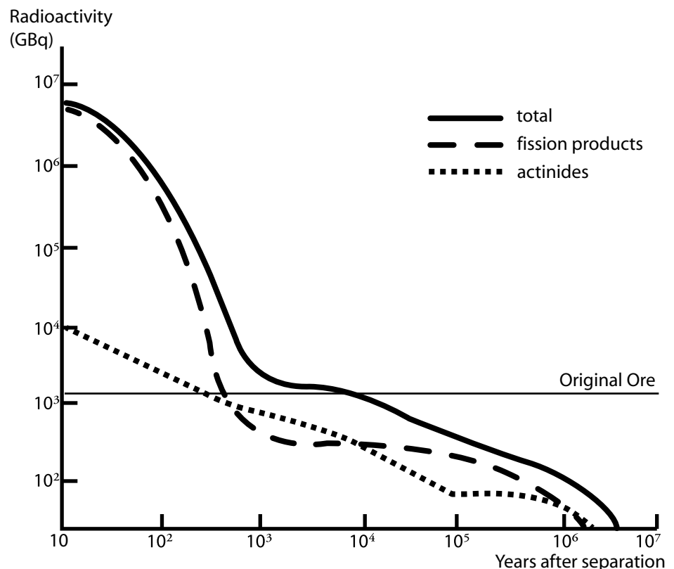
Figure 1: Decay in radioactivity of high-level waste from reprocessing one tonne of spent PWR fuel
